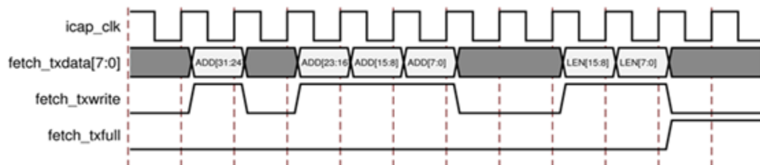
Figure 41: SEM Controller Sending Commands to Peripheral
