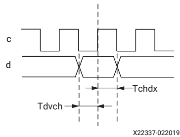
Figure 30: SPI Flash Device Input Data Capture Requirements
