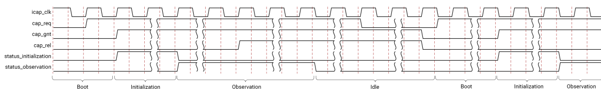
Figure 7: ICAP Arbitration Switching Behavior
