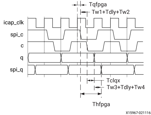
Figure 34: Output Data Capture Timing (Setup Analysis)
