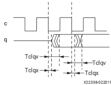
Figure 32: SPI Flash Device Output Data Switching Characteristics
