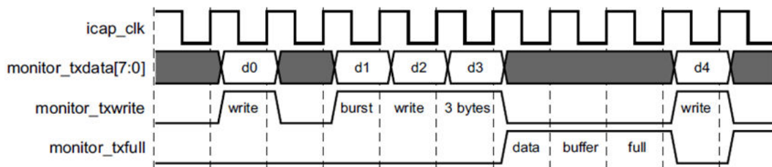
Figure 35: Monitor Interface Transmit Protocol
