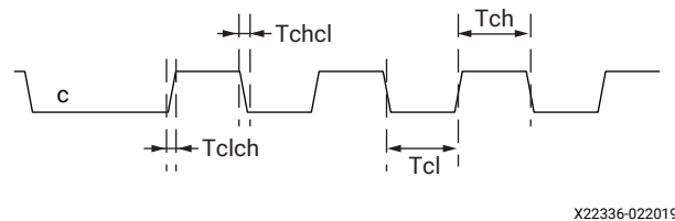
Figure 29: SPI Flash Device Input Clock Requirements
