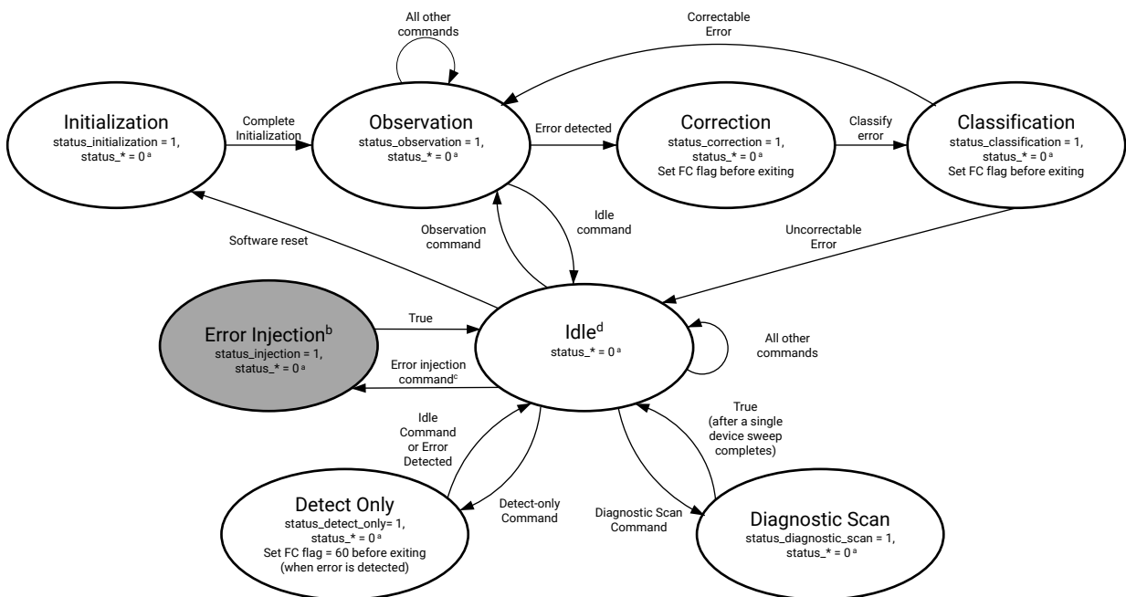
Figure 8: Valid State Transition Diagram for Mitigation Modes
