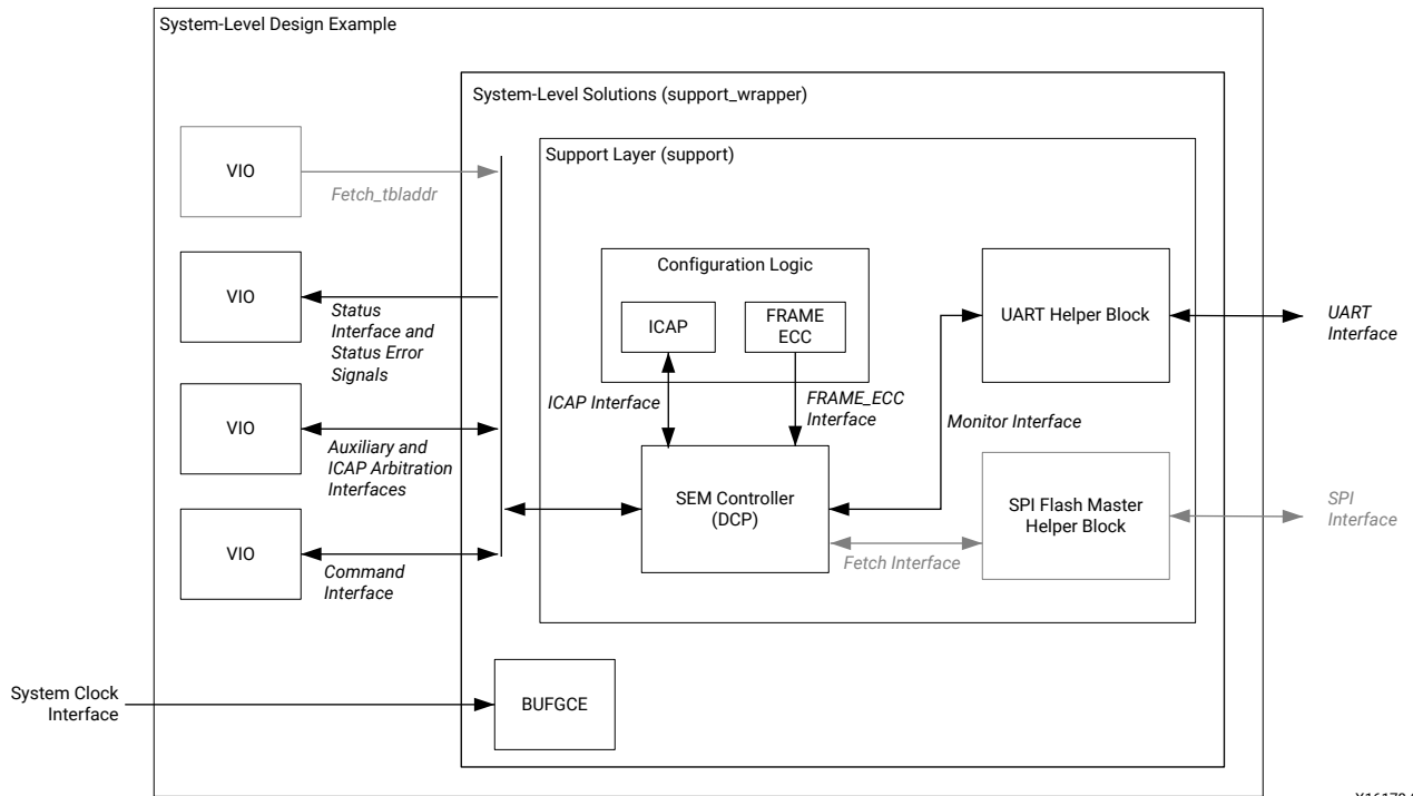
Figure 24: Example Design Block Diagram for Non-SSI Devices
