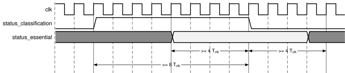
Figure 13: Status Interface Essential Flag Switching Characteristics (Mitigation Modes)
