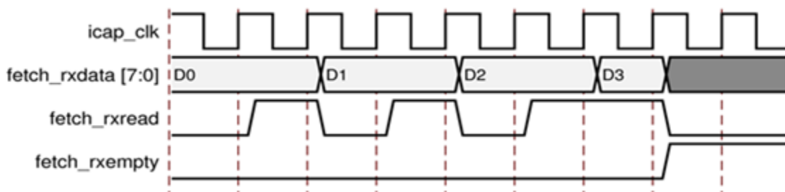
Figure 42: Peripheral Returning Data to SEM Controller
