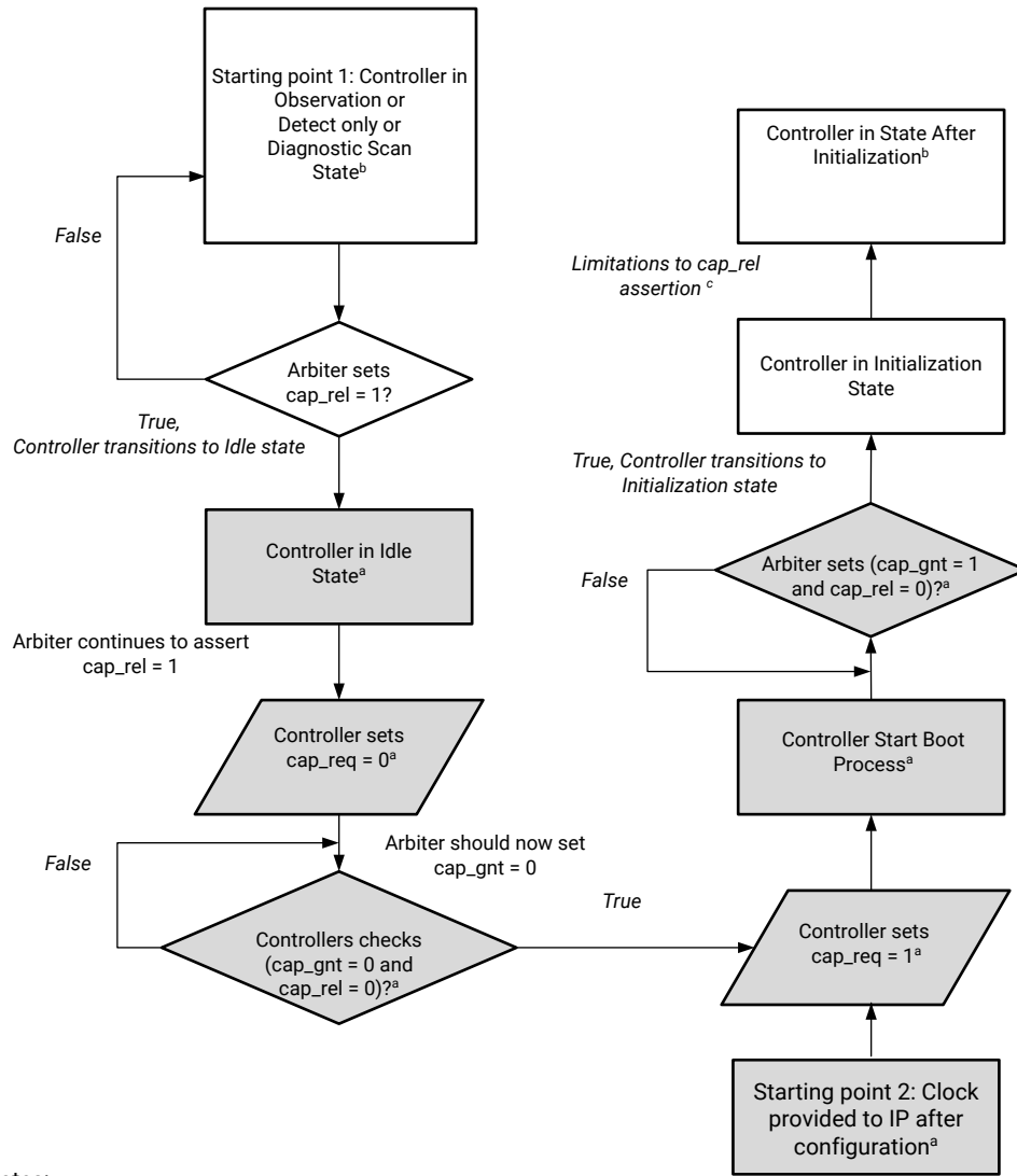
Figure 6: ICAP Arbitration Switching Behavior Flow Diagram
