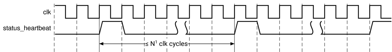
Figure 14: Status Interface Heartbeat Switching Characteristics
