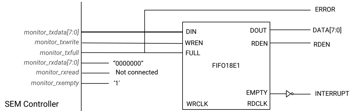
Figure 16: Connecting Monitor TX Interface to a FIFO
