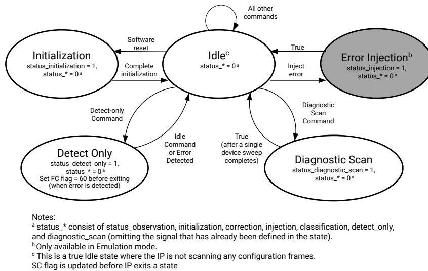
Figure 10: Valid State Transition Diagram for Other Modes
