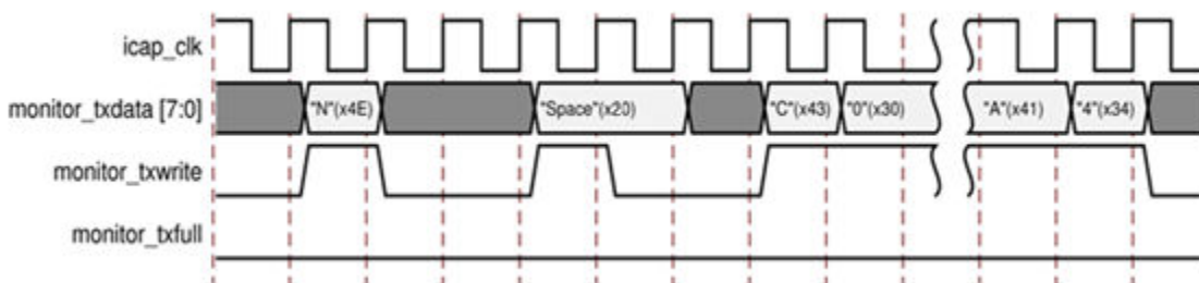
Figure 38: SEM Controller Receiving Error Injection Command from Peripheral Successfully
