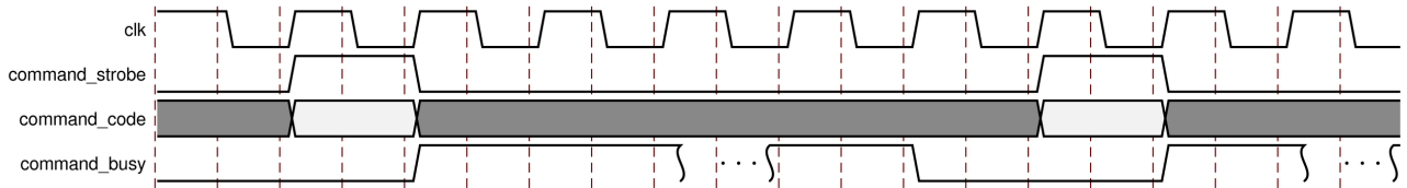
Figure 15: Command Interface Switching Behavior
