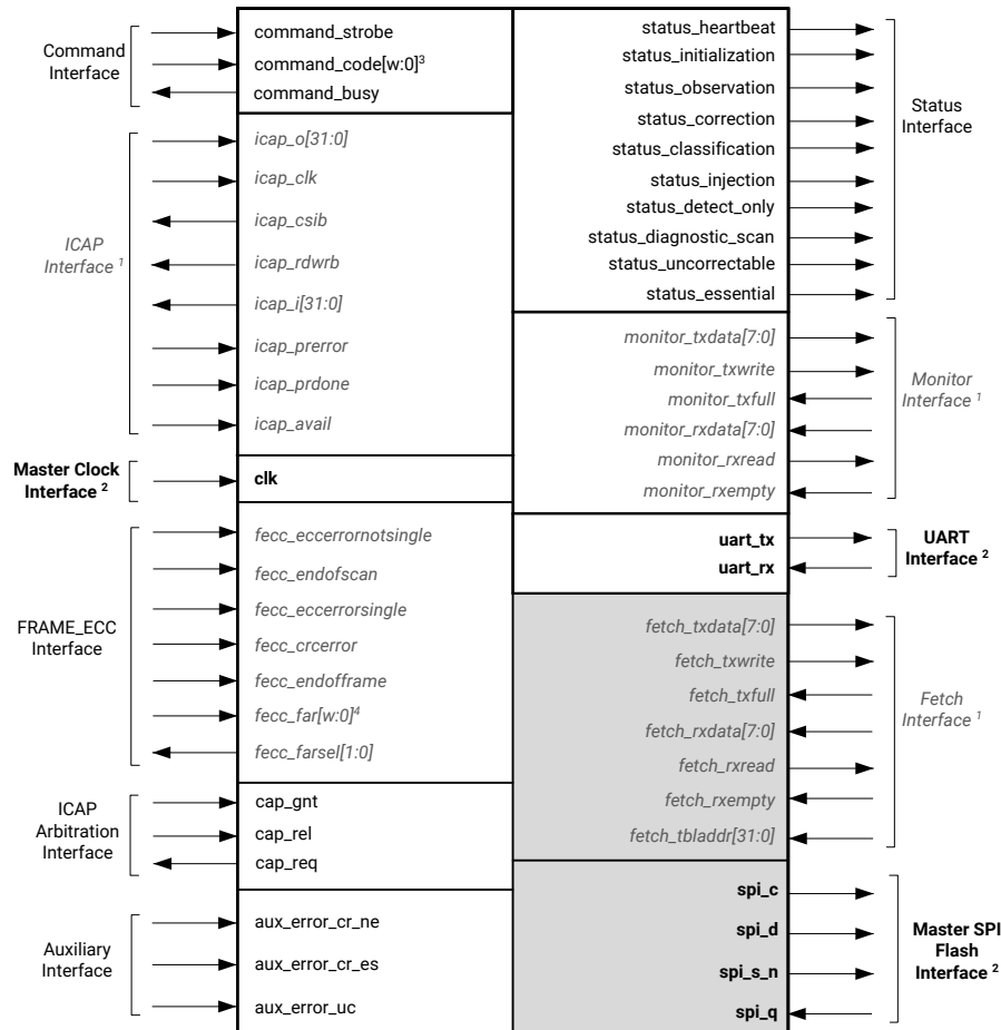
Figure 2: SEM Controller Ports for UltraScale and Monolithic UltraScale+ Devices
