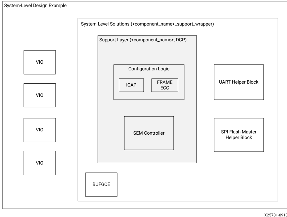
Figure 5: Configuration Primitive Included in Example Design
