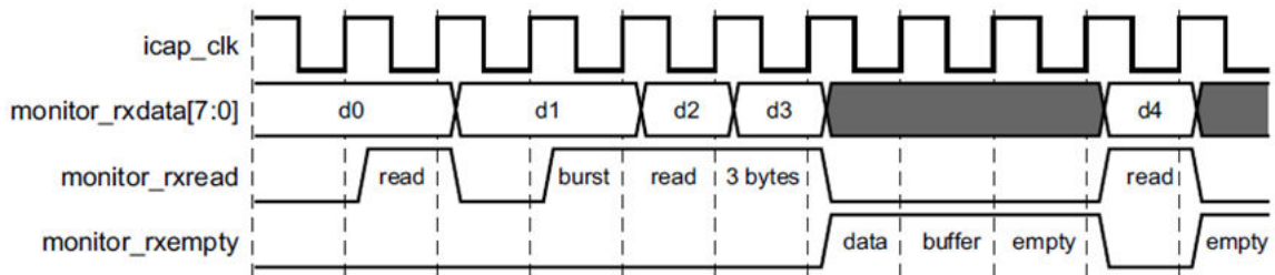
Figure 36: Monitor Interface Receive Protocol
