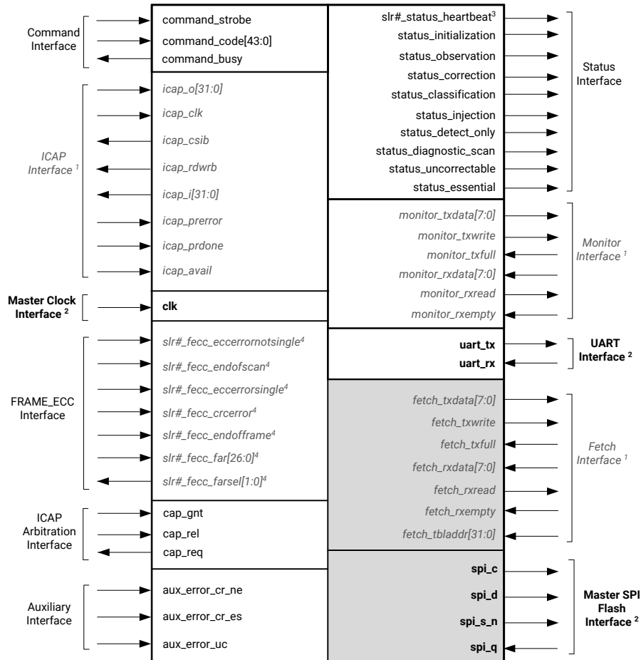
Figure 3: SEM Controller Ports for UltraScale+ SSI Devices
