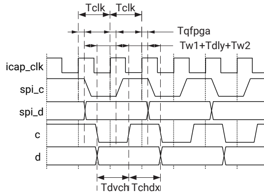
Figure 31: Input Data Capture Timing
