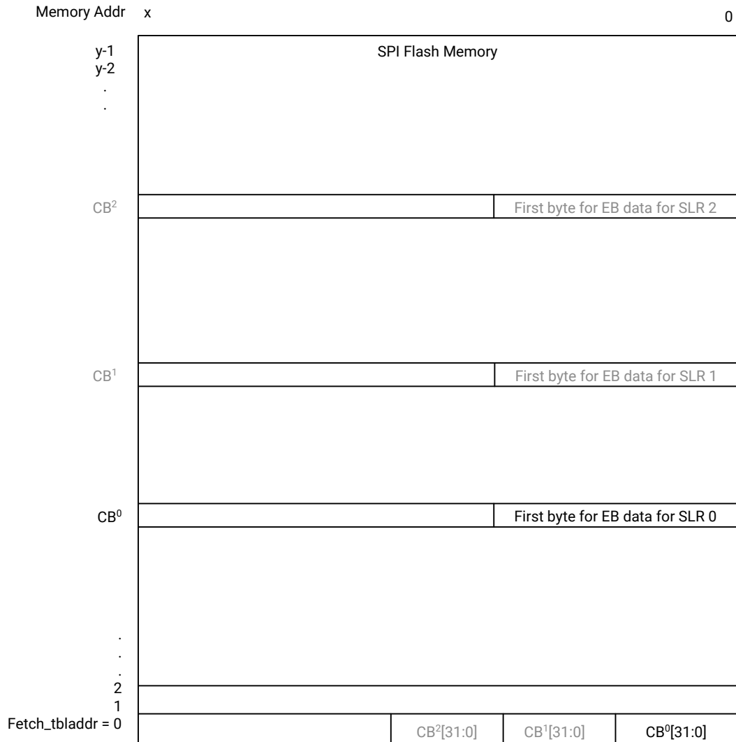
Figure 18: fetch_tbladdr Input Diagram
