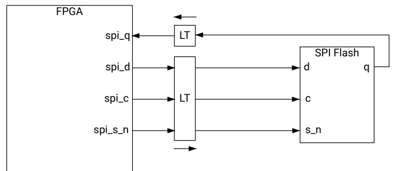
Figure 19: SPI Flash Device Connection, Including Level Translators
