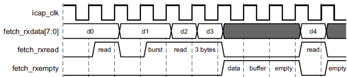
Figure 40: Fetch Interface Receive Protocol
