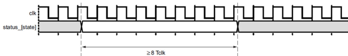
Figure 11: Status Interface State Signals Switching Characteristics
