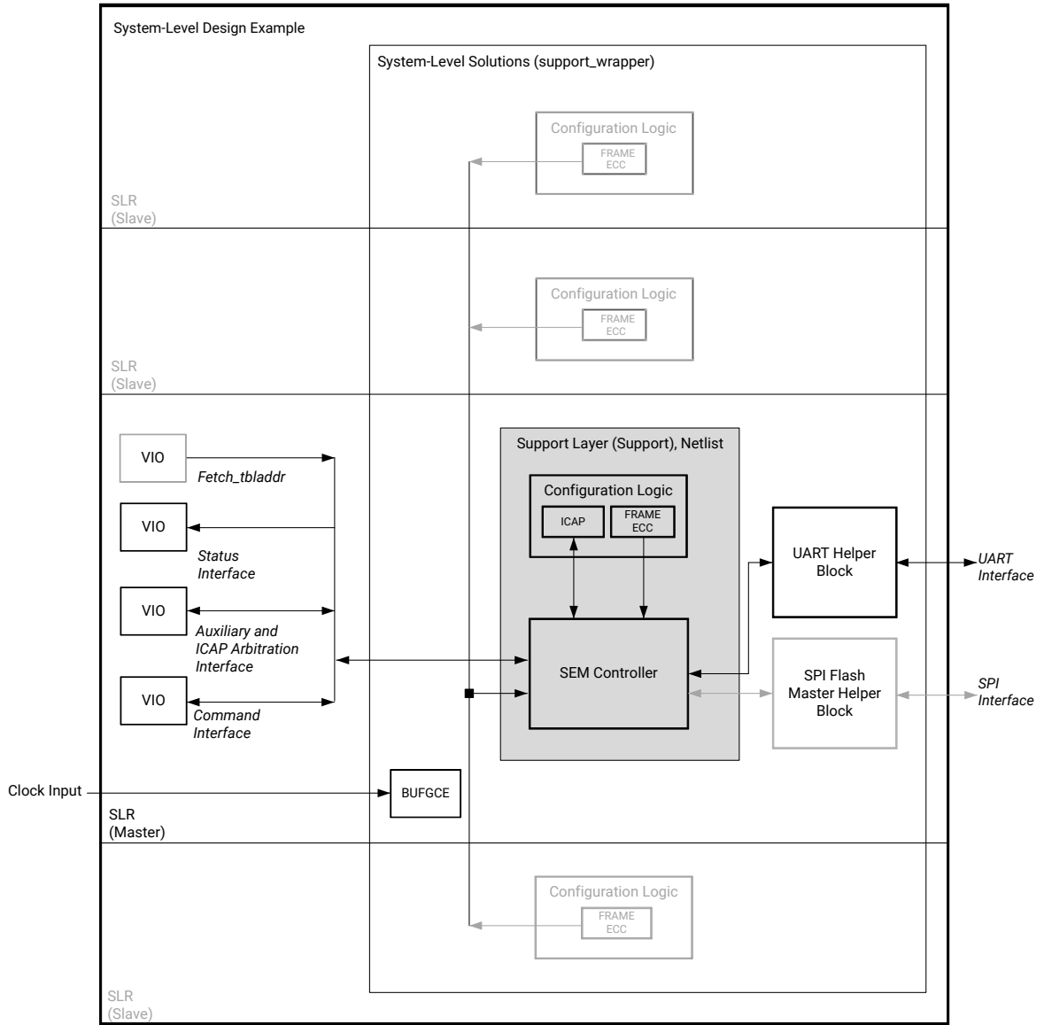
Figure 26: Example Design Block Diagram for UltraScale+ SSI Devices
