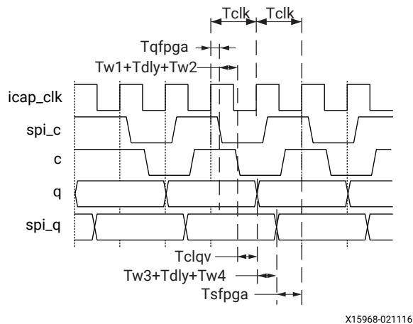
Figure 34: Output Data Capture Timing (Setup Analysis)
