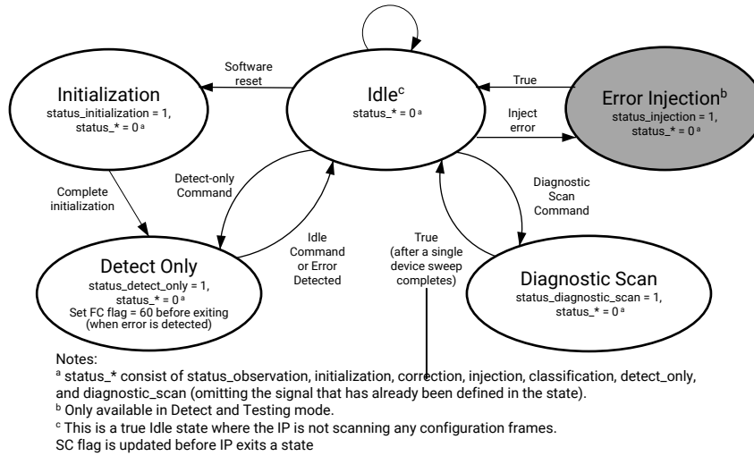
Figure 9: Valid State Transition Diagram for Detect Modes
