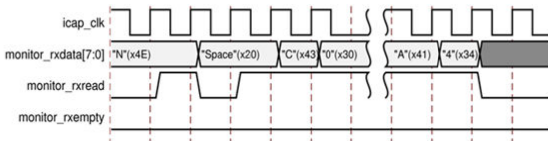
Figure 37: Peripheral Sending Error Injection Command Through Monitor RX Interface
