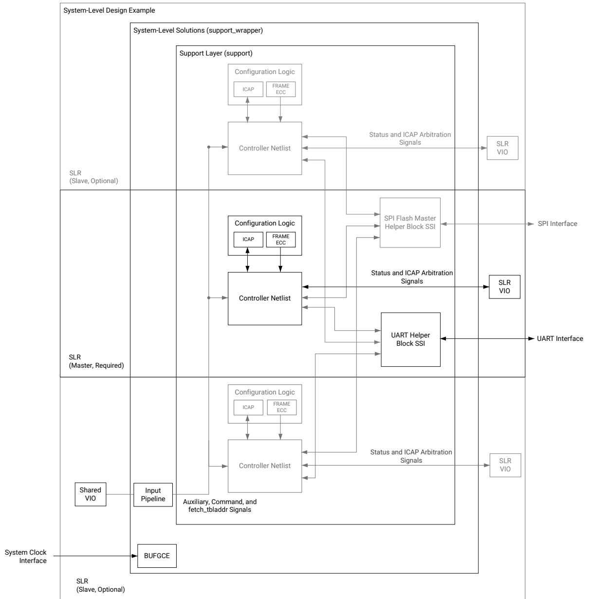
Figure 25: Example Design Block Diagram for UltraScale SSI Devices
