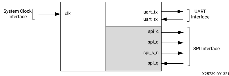
Figure 27: Example Design Ports
