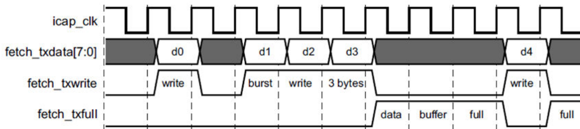
Figure 39: Fetch Interface Transmit Protocol
