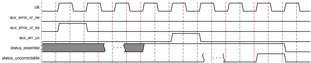
Figure 20: Switching Behavior for Auxiliary Interface
